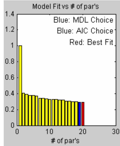
Figure 2 – Model fit vs model order (order 1 through order 20)
