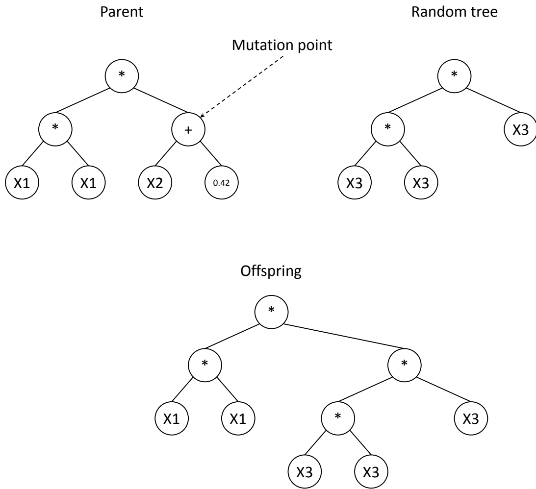
Figure 2.5: An example of a mutation operation
