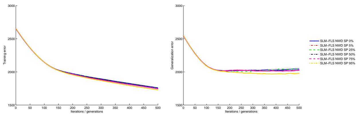
Figure 6.12: Training and generalization errors evolution plots for SLM-FLS NWD with and without sparseness
