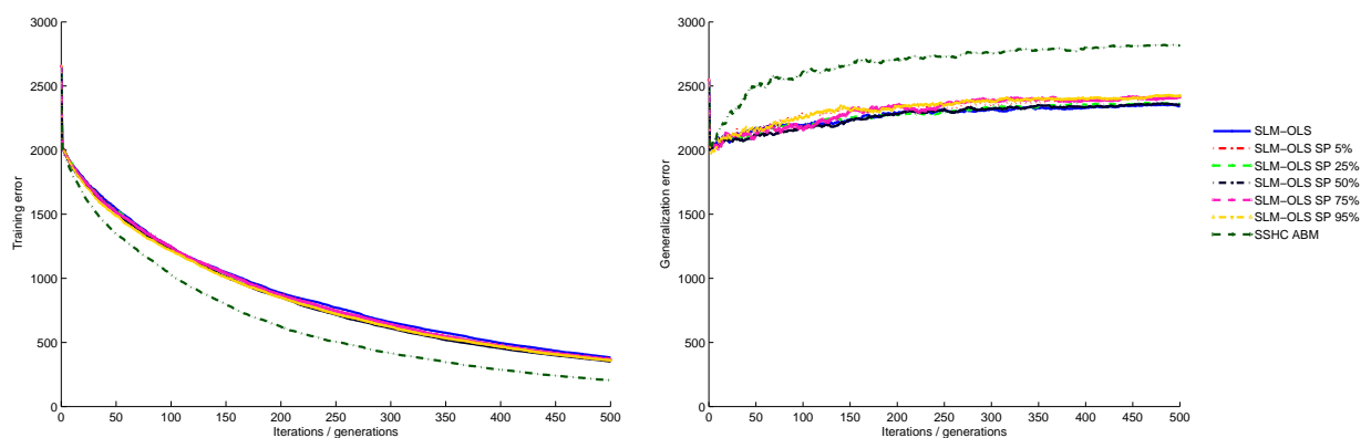
Figure 6.10: Training and generalization errors evolution plots for SLM-OLS with and without sparseness, and SSHC ABM
