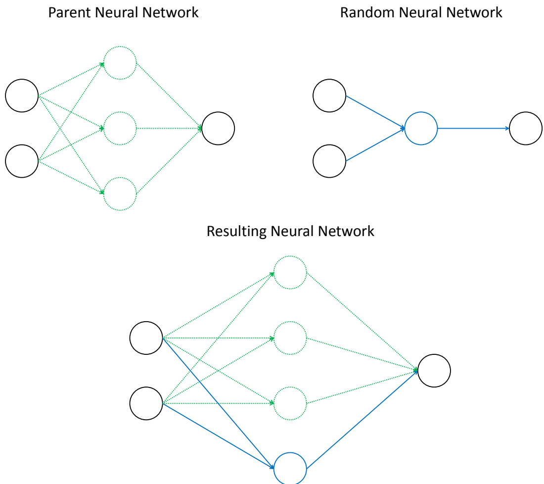
Figure 6.3: An example of an application of the GSM-NN operator
