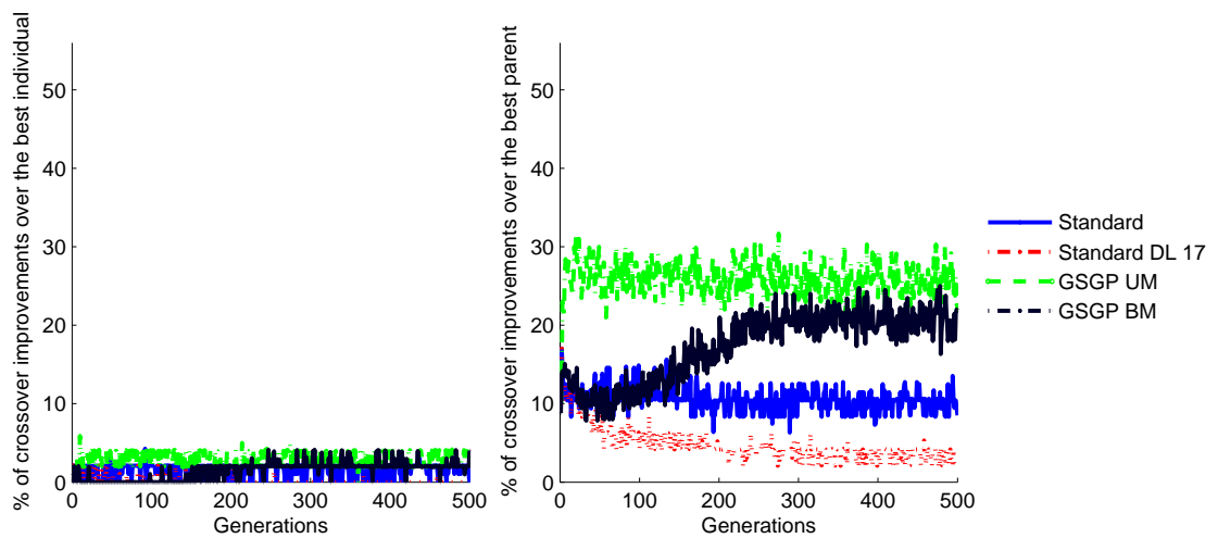
Figure 5.8: Percentage of crossover improvements for Standard GP and GSGP
