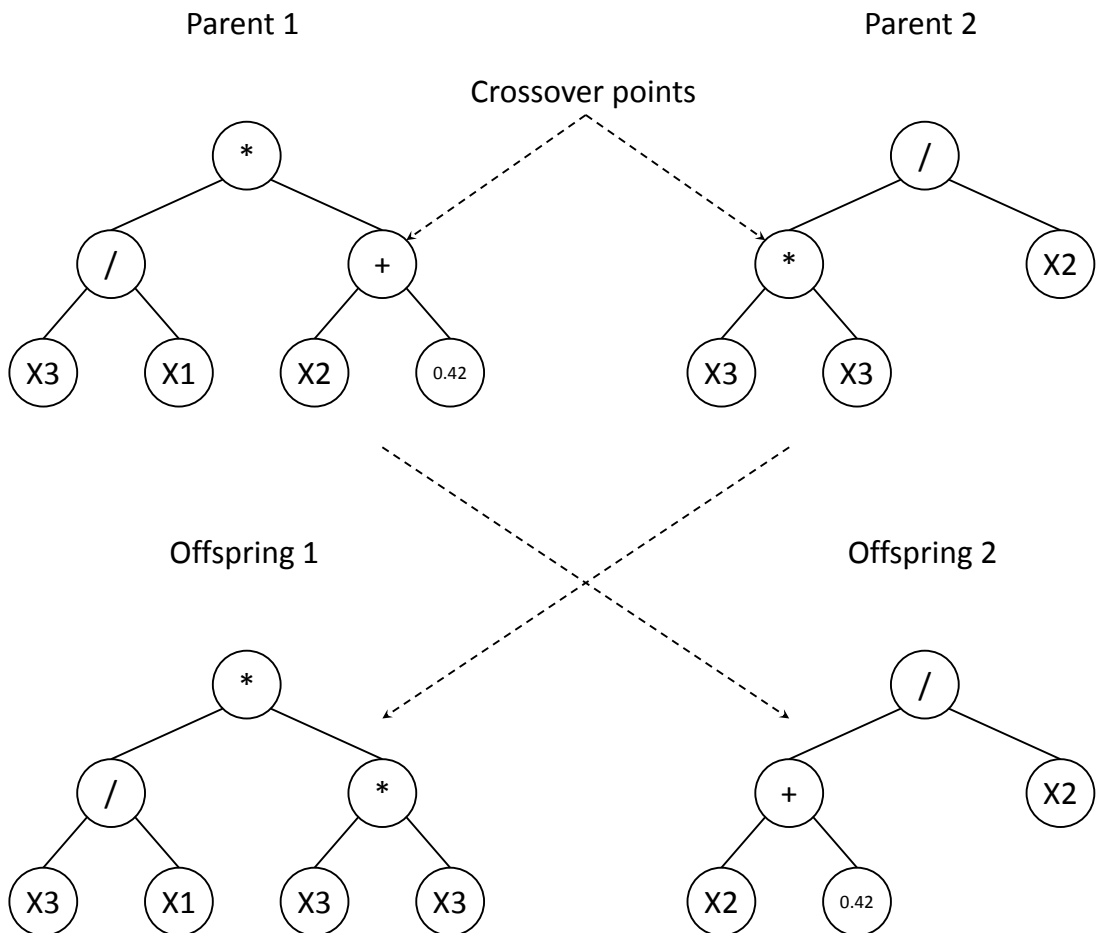
Figure 2.4: An example of a crossover operation
