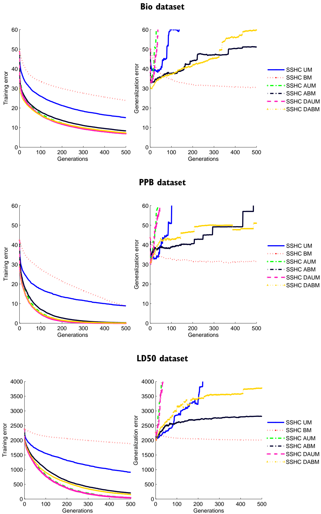
Figure 5.12: Training and generalization errors evolution plots for SSHC with and without adaptive mutation step
