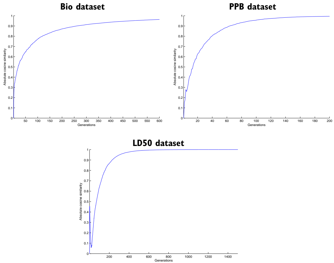
Figure 5.16: Absolute cosine similarity evolution for ACA-SSHC with k = 1.1
