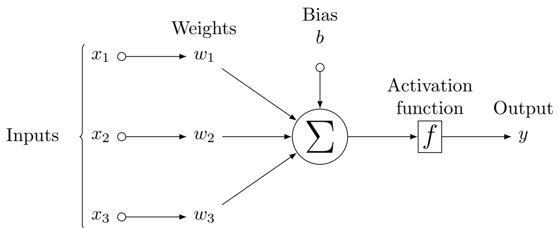
Figure 6.1: An artificial neuron with three inputs
