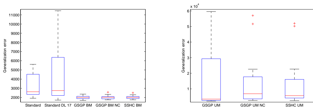
Figure 5.7: Generalization error boxplots for Standard GP, GSGP, and SSHC
