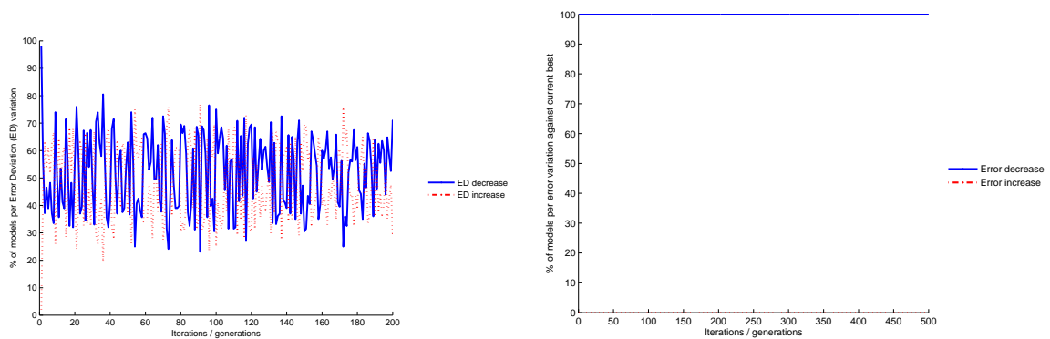
Figure 6.22: Evolution of the measures related to the EDV (left column) and the TIE (right column) criteria for SSHC ABM
