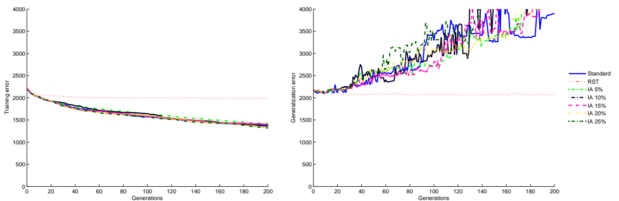
Figure 4.6: Training and generalization errors evolution plots for Standard GP, RST, and IA with different parameters
