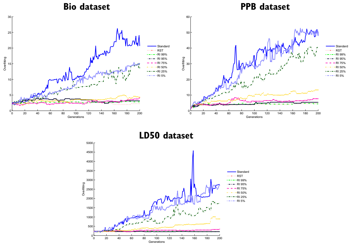
Figure 4.13: Overfitting evolution plots for Standard GP, RST, and RI with different parameters
