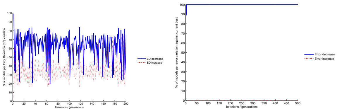
Figure 6.18: Evolution of the measures related to the EDV (left column) and the TIE (right column) criteria for SLM-OLS
