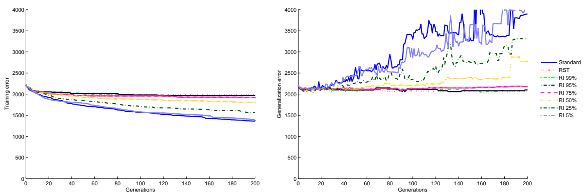
Figure 4.12: Training and generalization errors evolution plots for Standard GP, RST, and RI with different parameters
