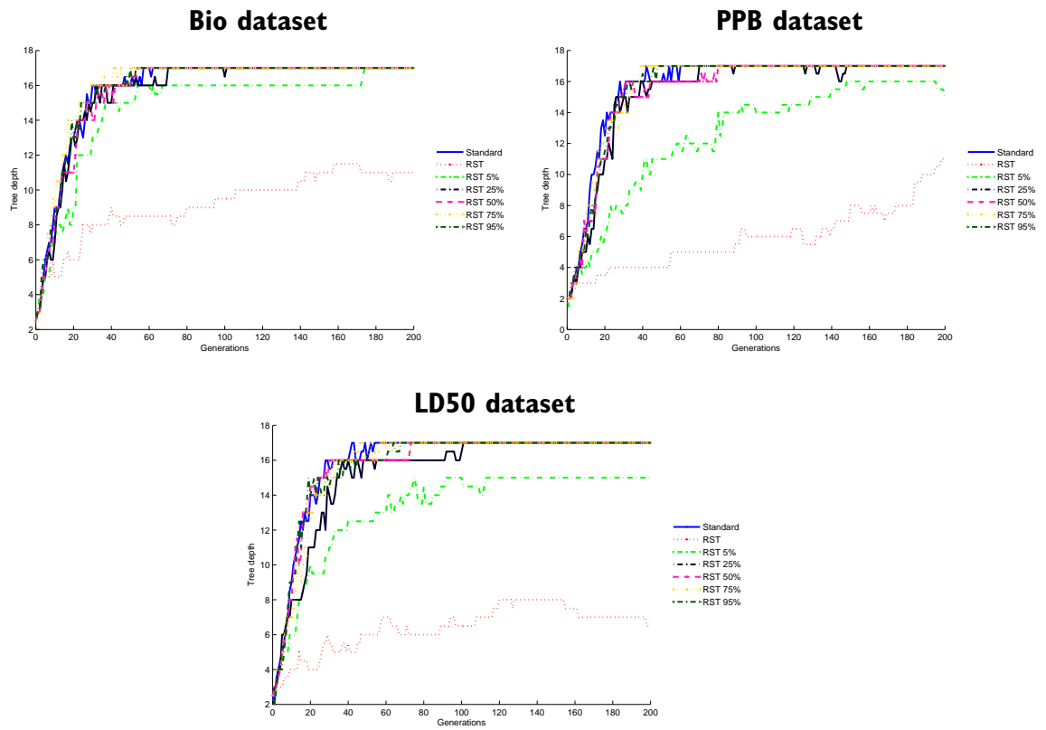
Figure 4.5: Tree depth evolution plots for Standard GP and RST with different parameters
