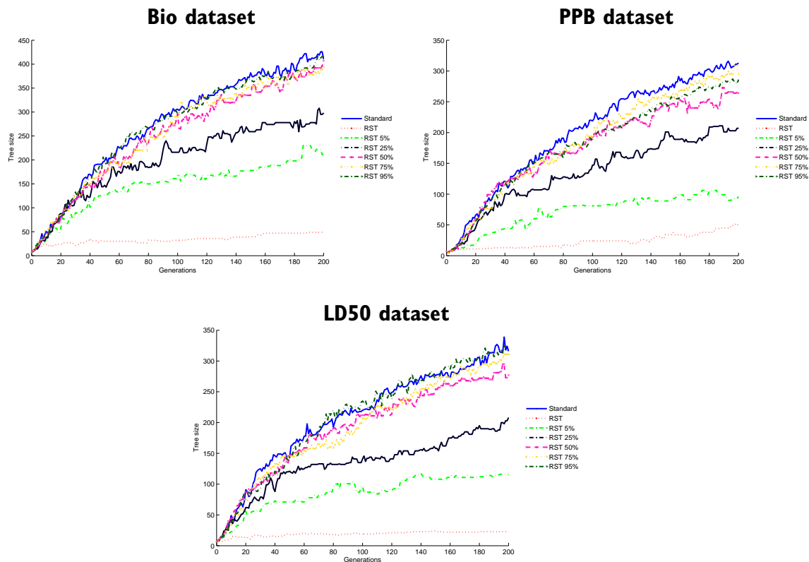
Figure 4.4: Tree size evolution plots for Standard GP and RST with different parameters
