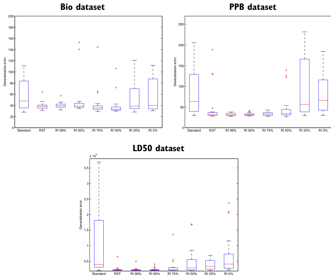
Figure 4.14: Generalization error boxplots for Standard GP, RST, and RI with different parameters
