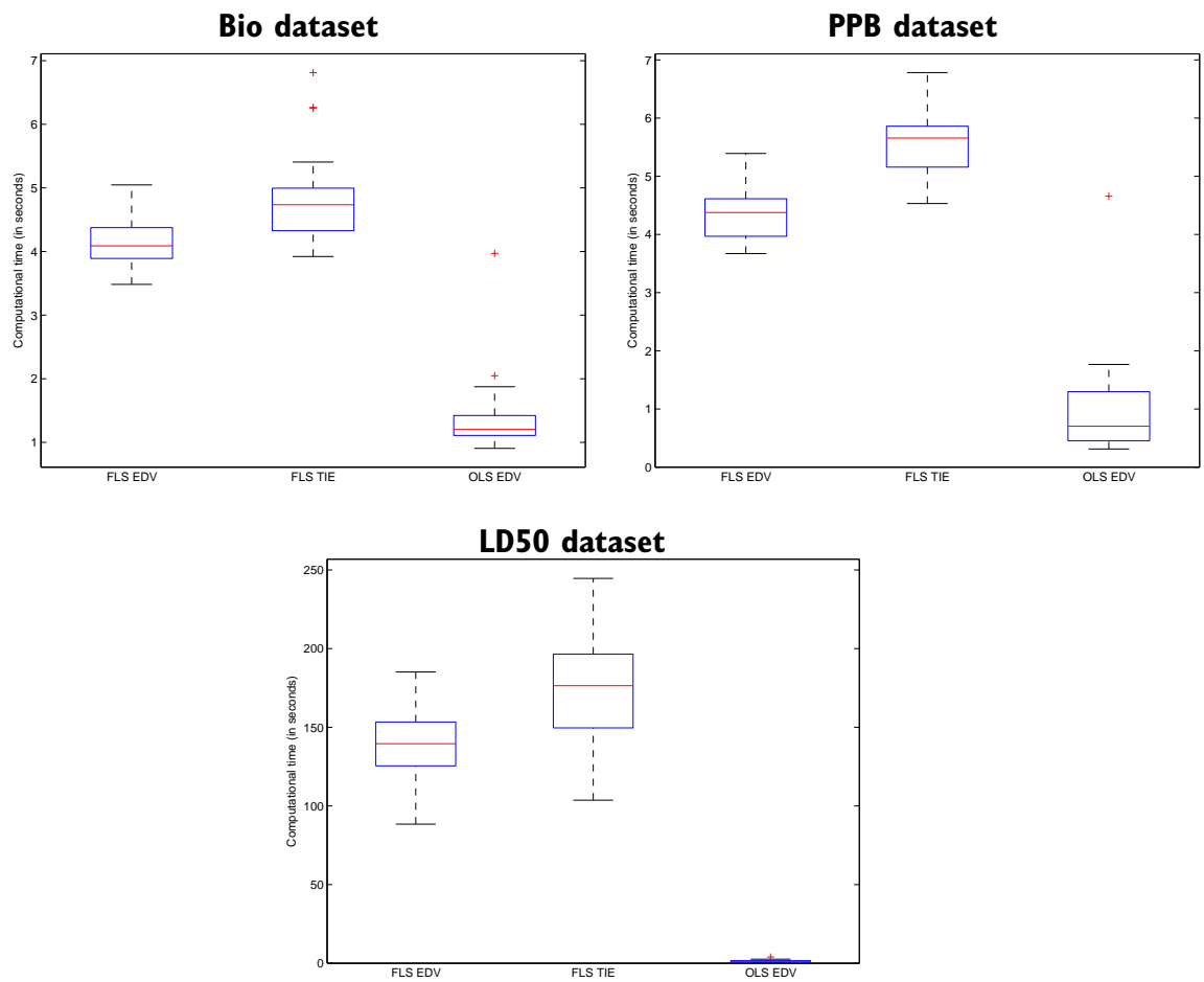
Figure 6.25: Computational time of each SLM variant
