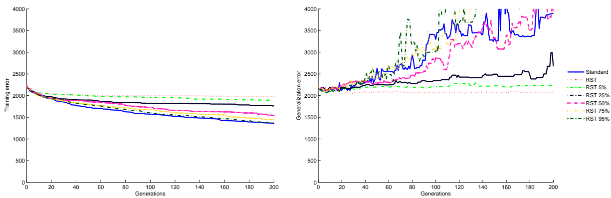
Figure 4.1: Training and generalization errors evolution plots for Standard GP and RST with different parameters
