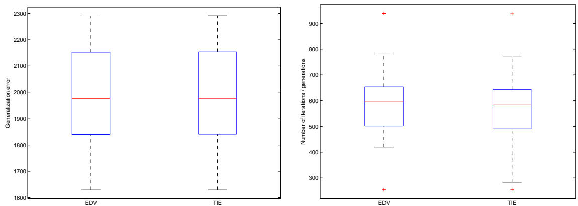
Figure 6.17: Boxplots with the generalization errors (left column) and the number of iterations (right column) resulting from the application of both stopping criteria with a 25% stopping threshold to SLM-FLS
