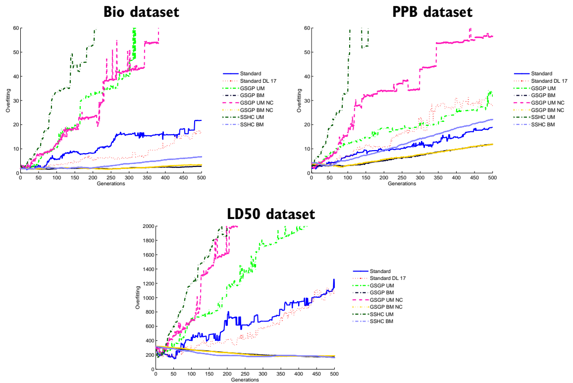
Figure 5.6: Overfitting evolution plots for Standard GP, GSGP, and SSHC
