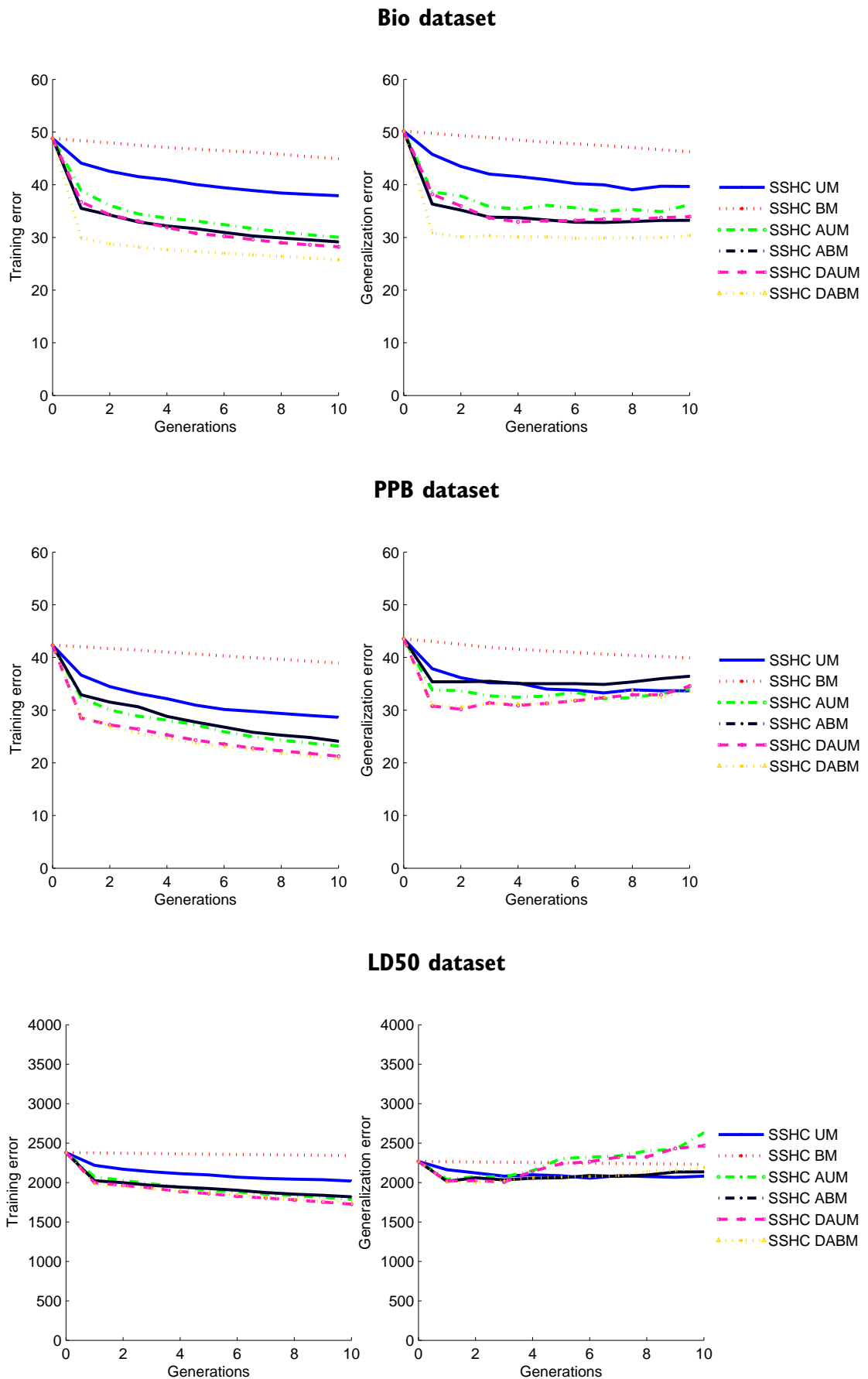
Figure 5.13: Training and generalization errors evolution plots for the first 10 generations for SSHC with and without adaptive mutation step
