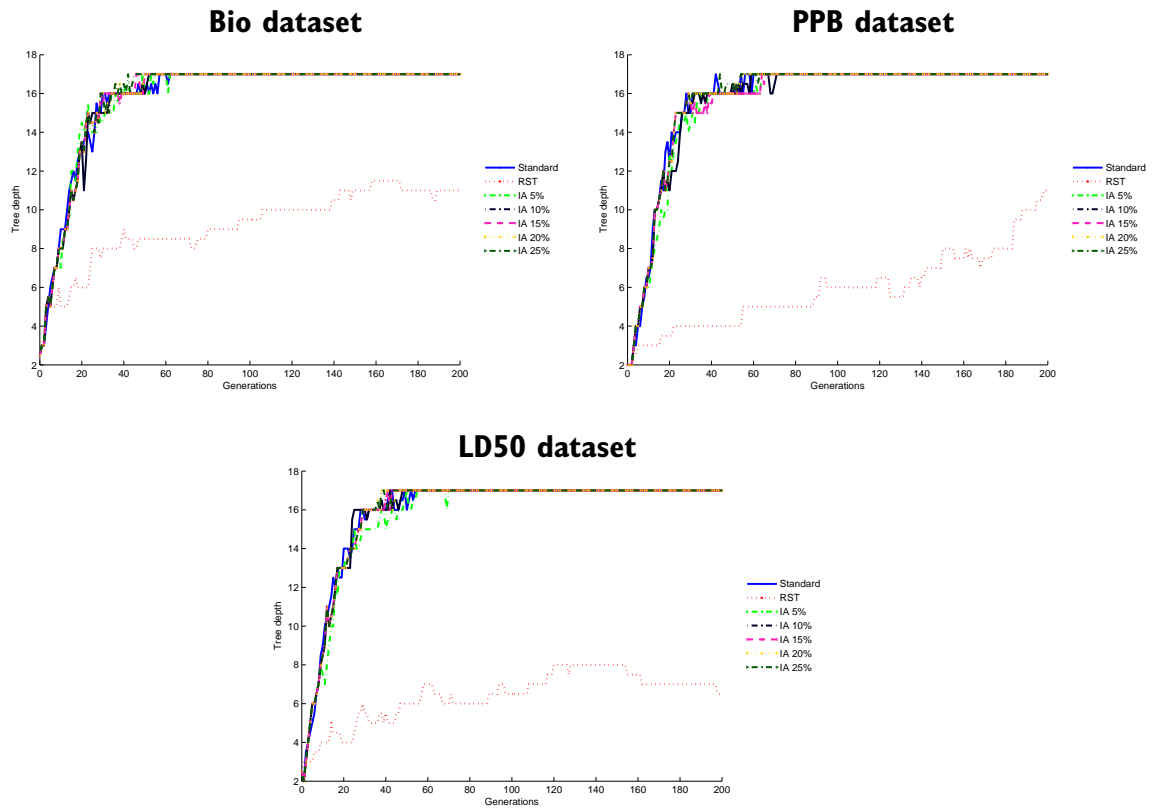
Figure 4.8: Tree depth evolution plots for Standard GP, RST, and IA with different parameters
