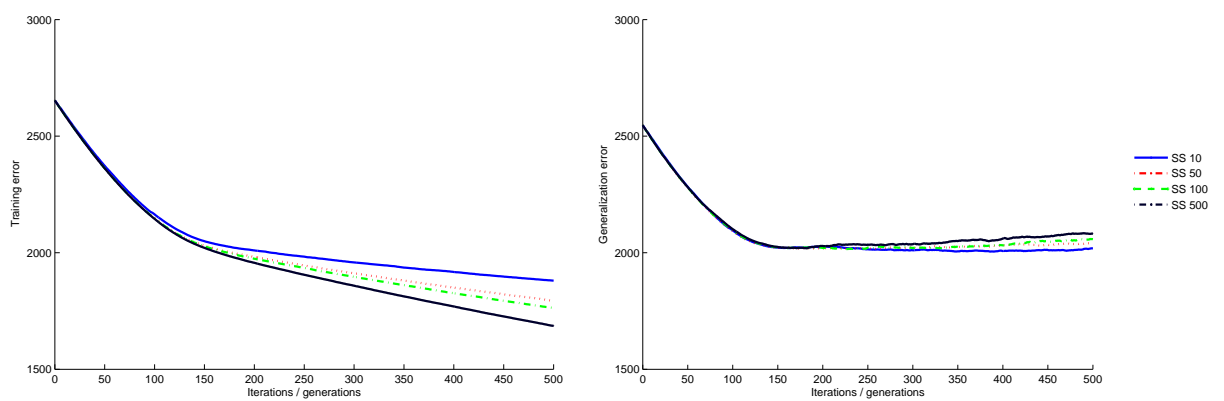
Figure 6.5: Training and generalization errors evolution plots for SLM with different sample sizes
