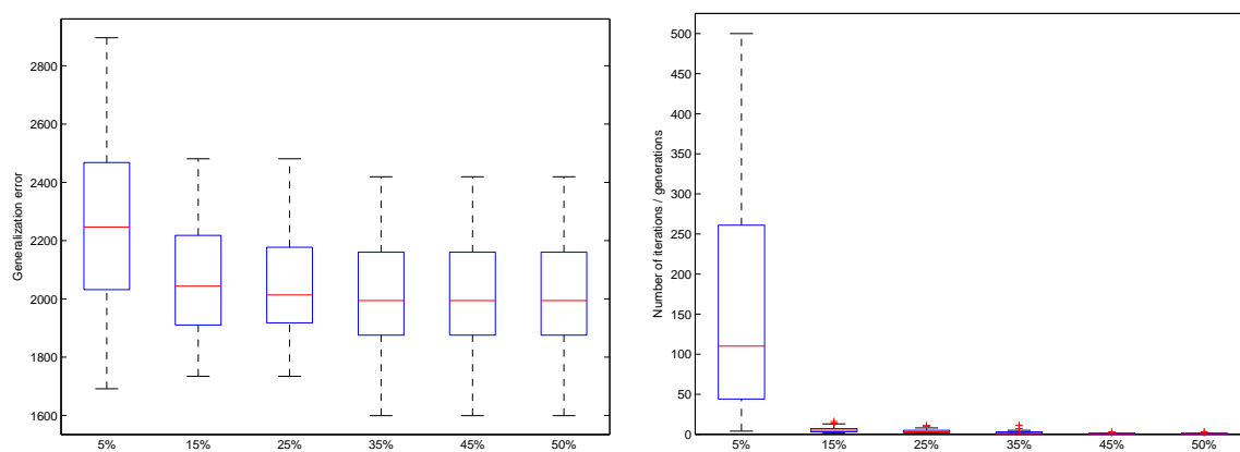
Figure 6.19: Boxplots with the generalization errors (left column) and the number of iterations (right column) resulting from the application of the EDV criterion with different stopping thresholds to SLM-OLS
