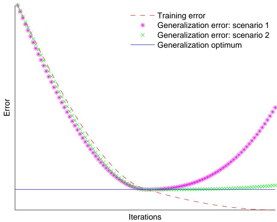
Figure 2.1: Typical evolutions of the training and generalization errors of an iterative supervised learning method across its iterations
