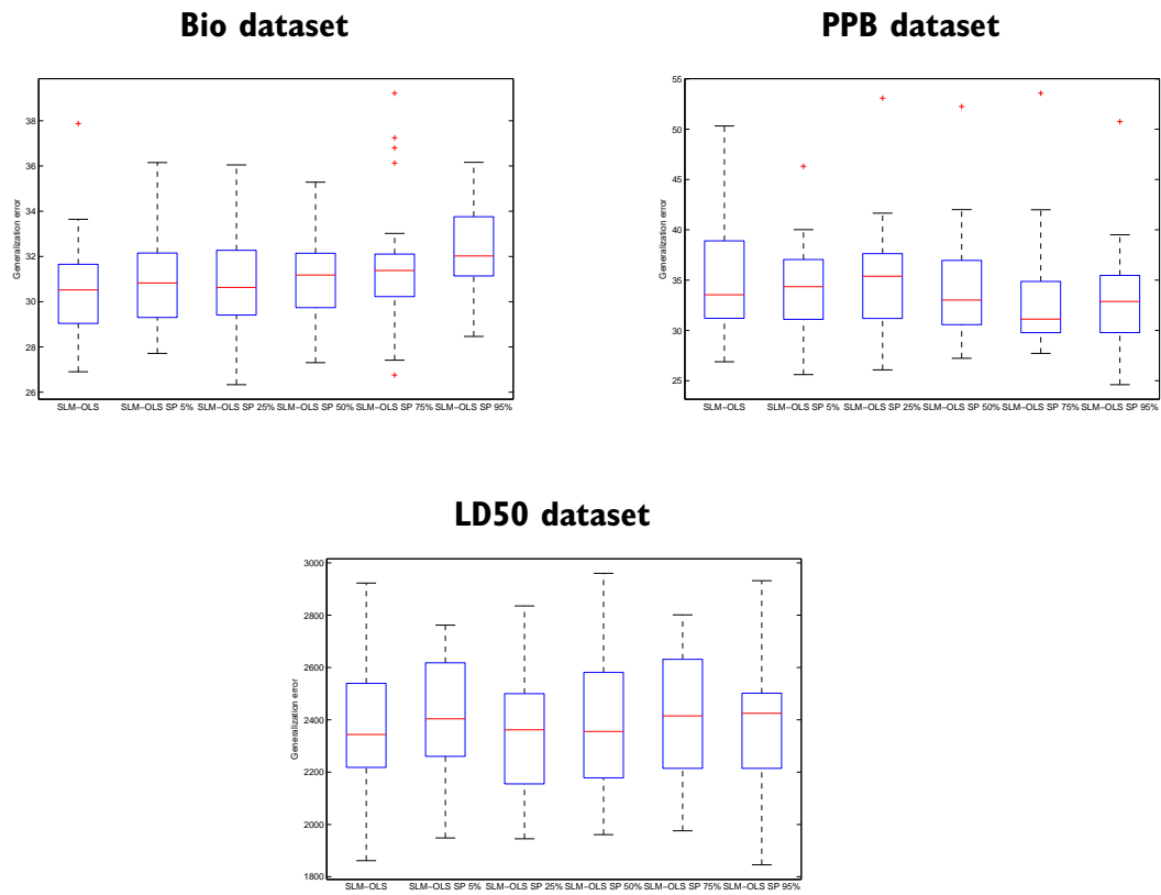
Figure 6.11: Generalization error boxplots for SLM-OLS with and without sparseness
