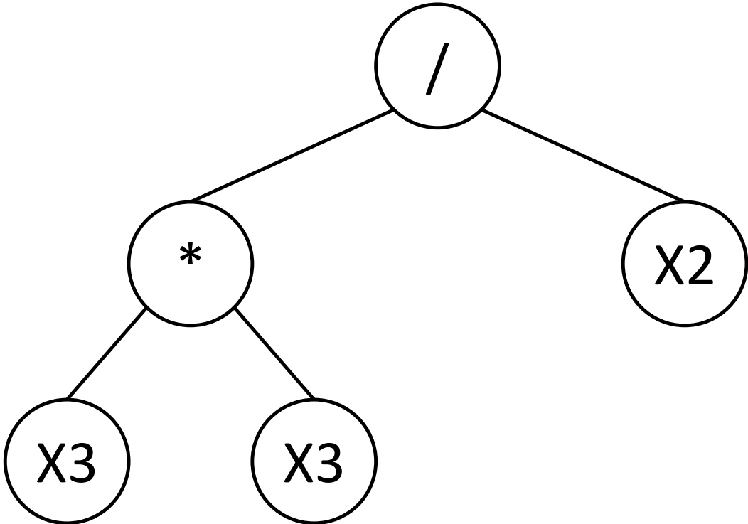
Figure 2.3: A GP individual that represents the function X3^2/X2
