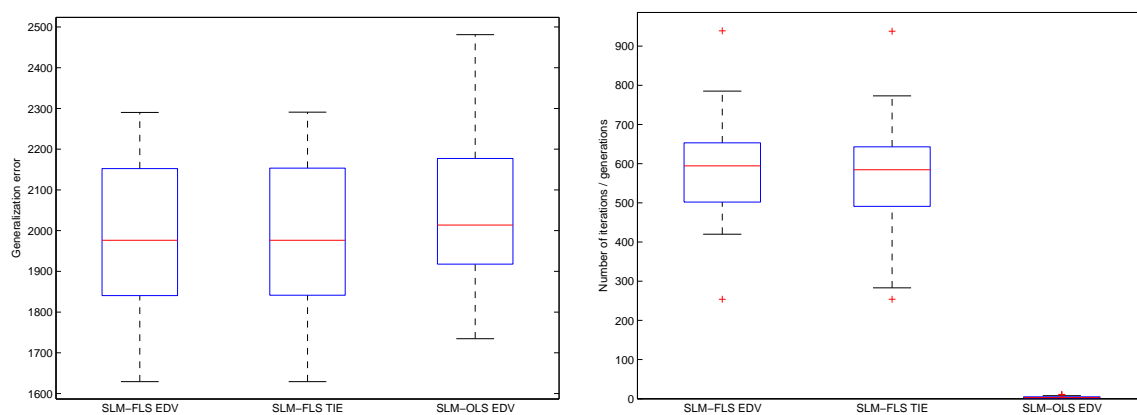
Figure 6.20: Boxplots with the generalization errors (left column) and the number of iterations (right column) resulting from the application of both stopping criteria with a 25% stopping threshold to SLM-FLS and SLM-OLS
