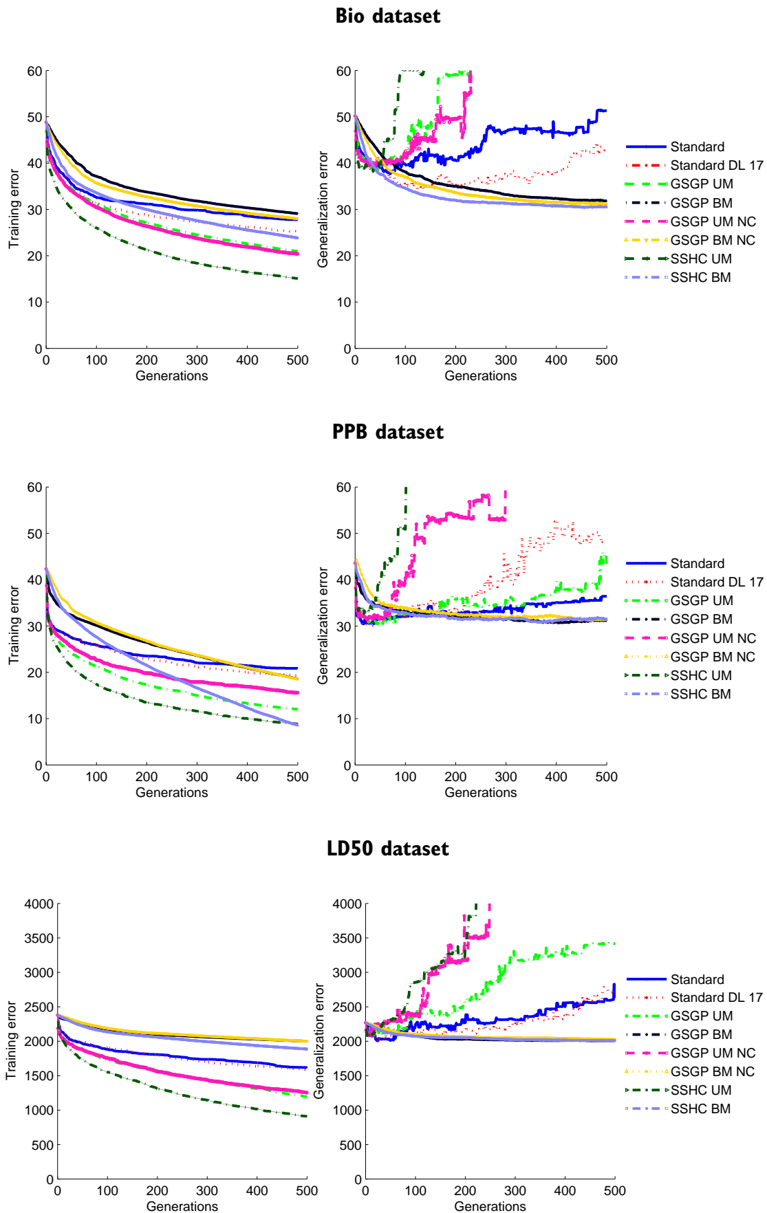
Figure 5.5: Training and generalization errors evolution plots for Standard GP, GSGP, and SSHC
