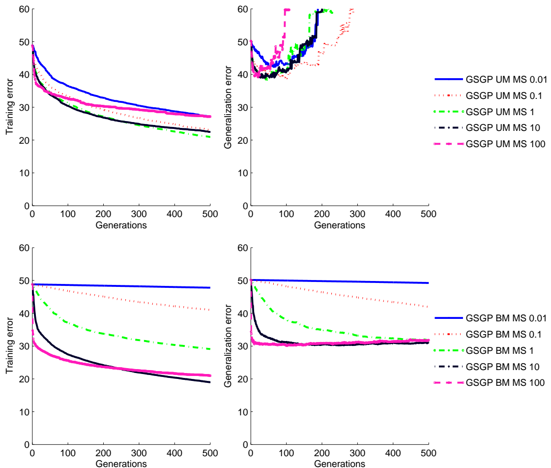
Figure 5.1: Training and generalization errors evolution plots for GSGP UM (top) and BM (bottom), with several mutation steps in the Bio dataset
