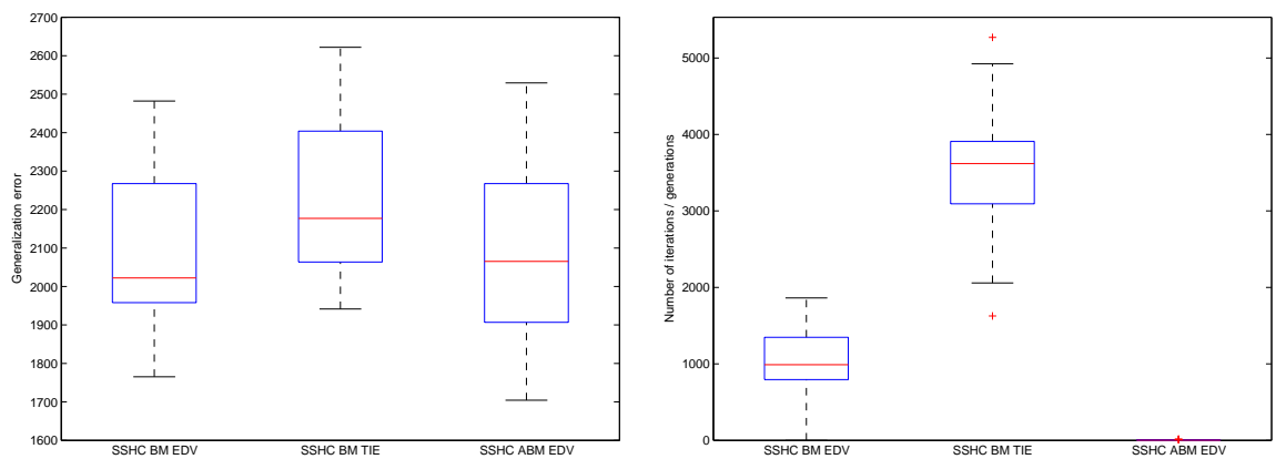
Figure 6.23: Boxplots with the generalization errors (left column) and the number of generations (right column) resulting from the application of both stopping criteria with a 25% stopping threshold to SSHC BM and SSHC ABM
