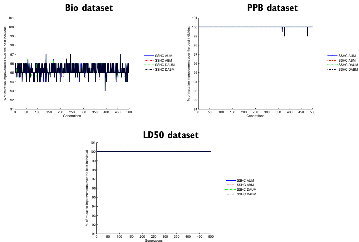
Figure 5.14: Percentage of mutation improvements for SSHC with adaptive mutation step
