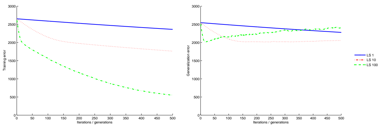
Figure 6.4: Training and generalization errors evolution plots for SLM with different learning steps
