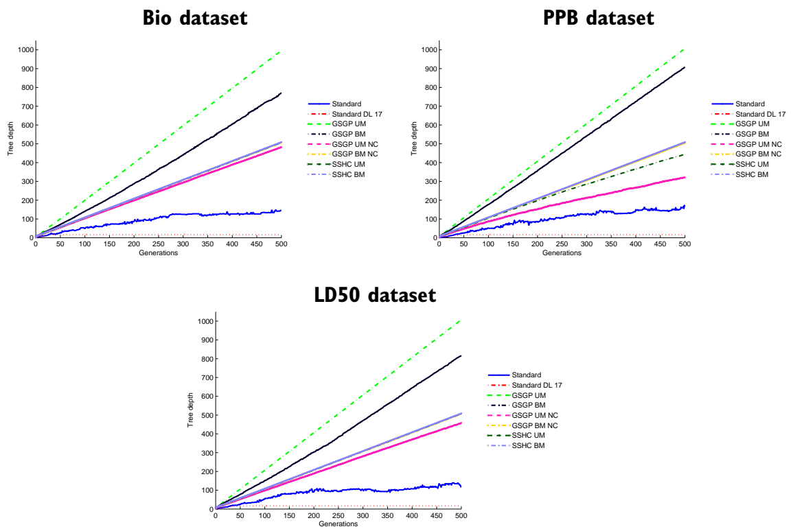
Figure 5.11: Tree depth evolution plots for Standard GP, GSGP, and SSHC
