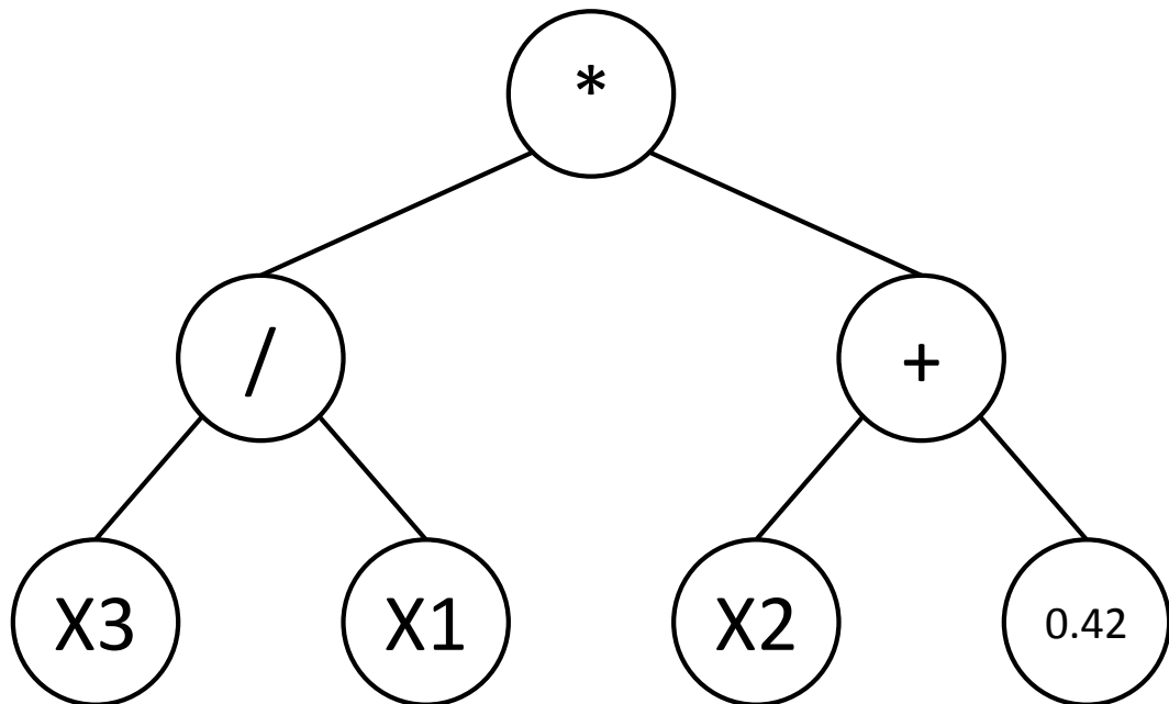
Figure 2.2: A GP individual that represents the function X3/X1 * (X2 + 0.42)
