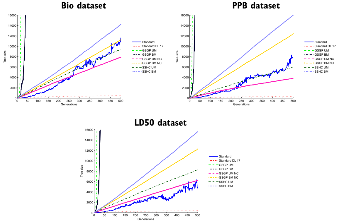
Figure 5.10: Tree size evolution plots for Standard GP, GSGP, and SSHC
