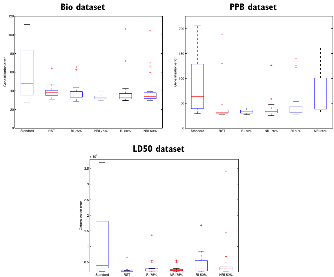
Figure 4.17: Generalization error boxplots for Standard GP, RST, RI 50% and 75%, and NRI 50% and 75%
