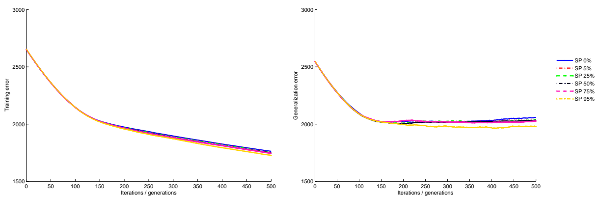
Figure 6.6: Training and generalization errors evolution plots for SLM with and without sparseness
