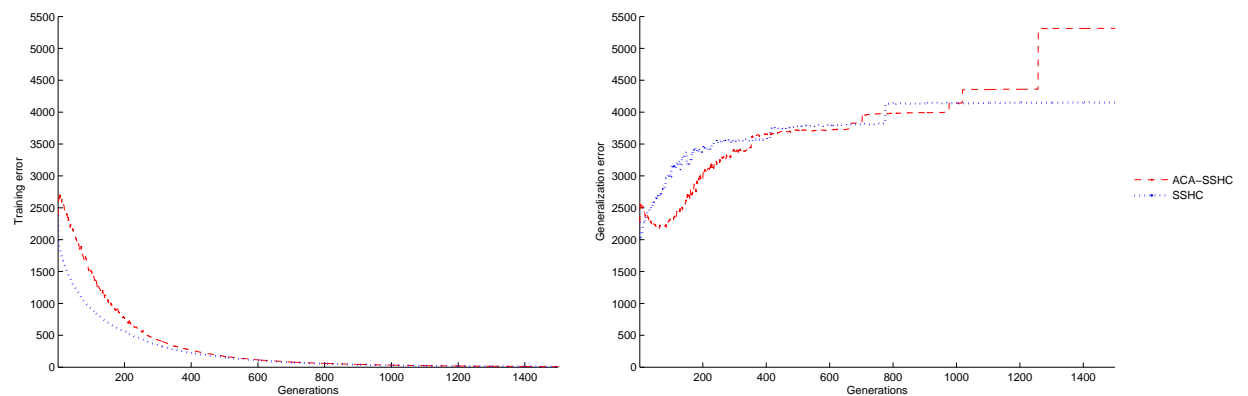
Figure 5.17: Training and generalization errors evolution plots for ACA-SSHC with k = 1.1 and SSHC
