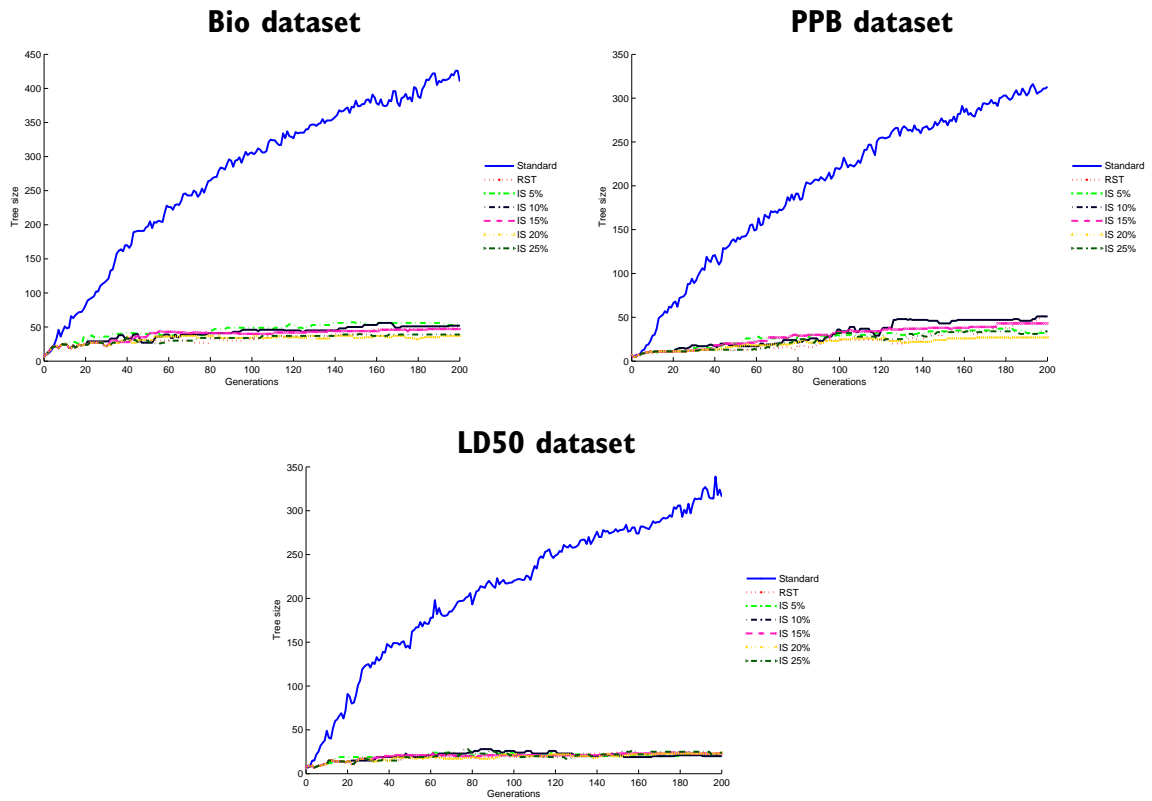
Figure 4.10: Tree size evolution plots for Standard GP, RST, and IS with different parameters
