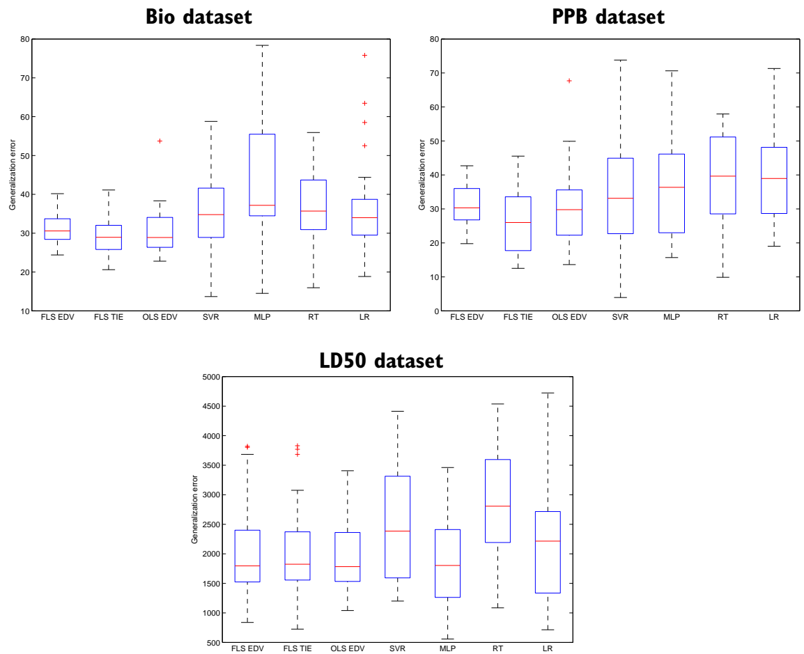
Figure 6.24: Boxplots with the generalization errors across the 30 folds
