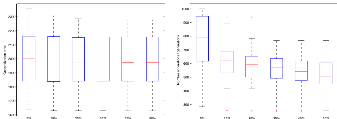
Figure 6.15: Boxplots with the generalization errors (left column) and the number of iterations (right column) resulting from the application of the EDV criterion with different stopping thresholds to SLM-FLS
