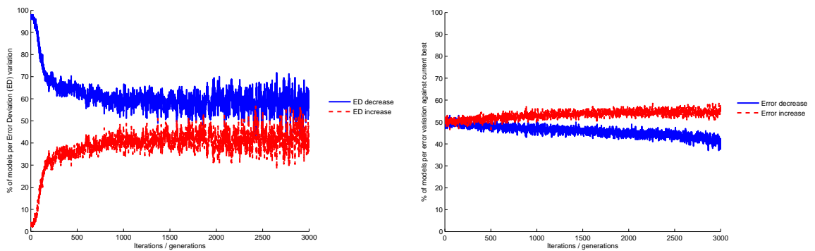
Figure 6.21: Evolution of the measures related to the EDV (left column) and the TIE (right column) criteria for SSHC BM
