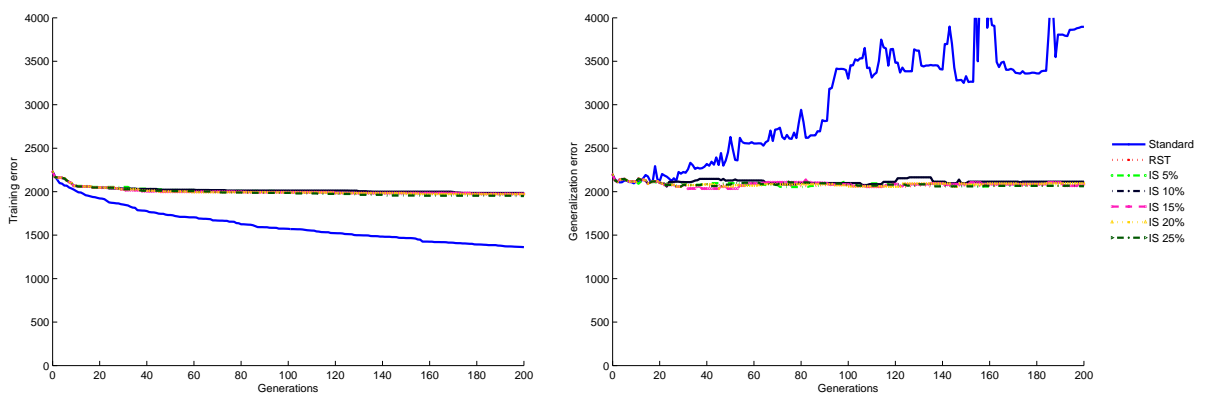
Figure 4.9: Training and generalization errors evolution plots for Standard GP, RST, and IS with different parameters
