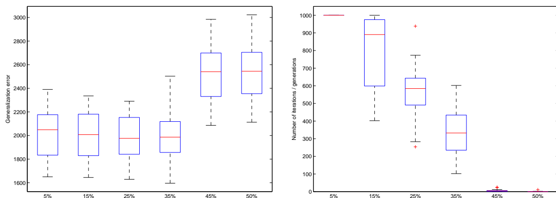
Figure 6.16: Boxplots with the generalization errors (left column) and the number of iterations (right column) resulting from the application of the TIE criterion with different stopping thresholds to SLM-FLS
