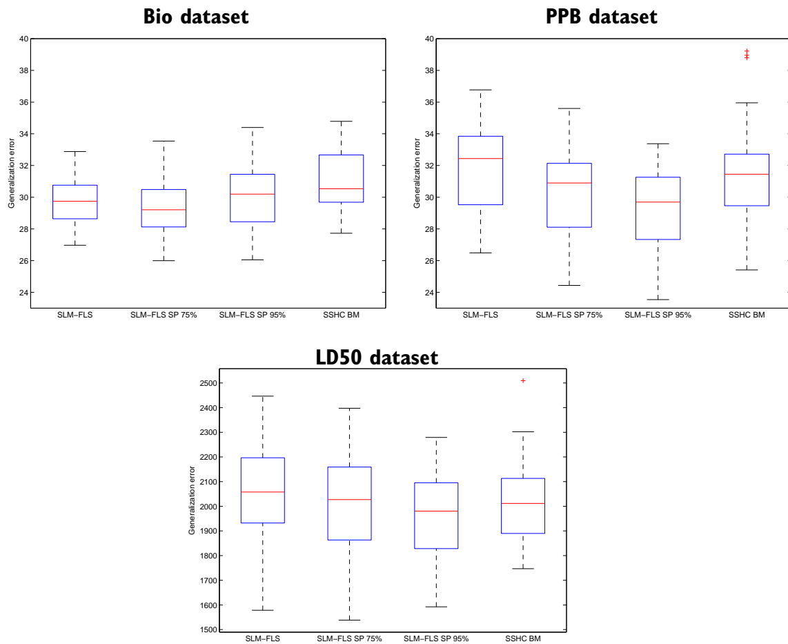
Figure 6.9: Generalization error boxplots for SLM-FLS, SLM-FLS SP 75%, SLM-FLS SP 95%, and SSHC BM
