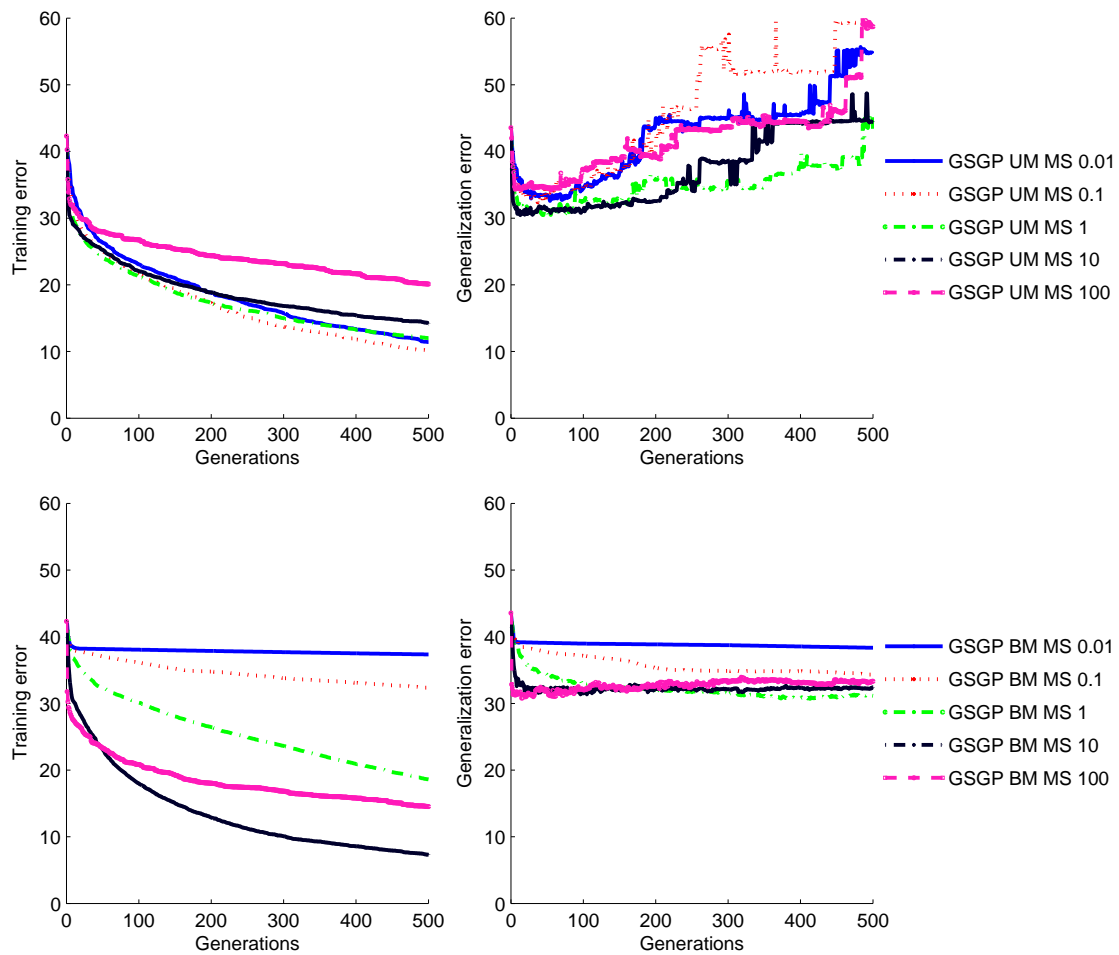
Figure 5.2: Training and generalization errors evolution plots for GSGP UM (top) and BM (bottom), with several mutation steps in the PPB dataset
