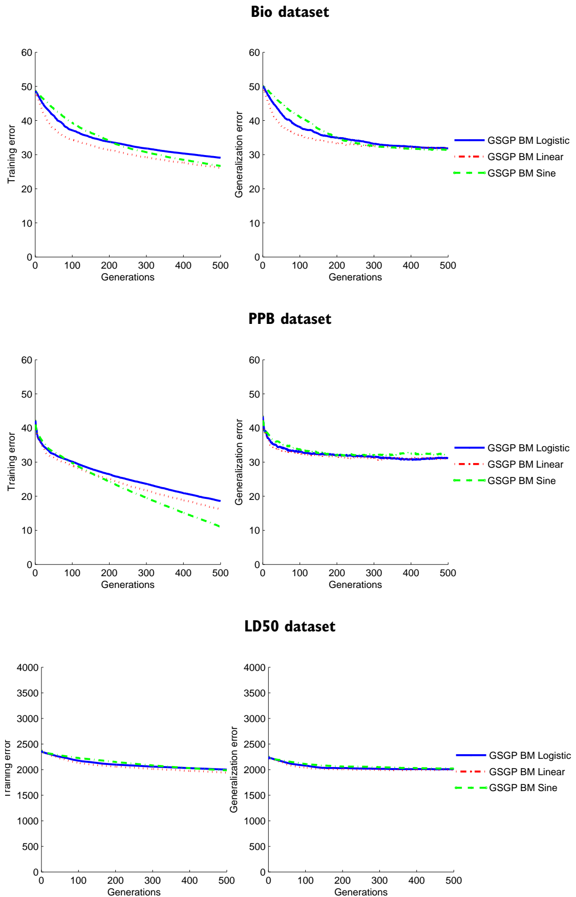
Figure 5.4: Training and generalization errors evolution plots for GSGP BM with different bounding functions
