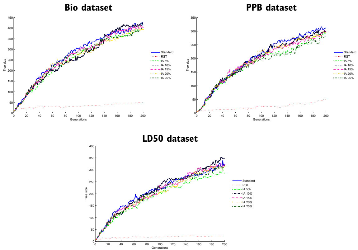
Figure 4.7: Tree size evolution plots for Standard GP, RST, and IA with different parameters
