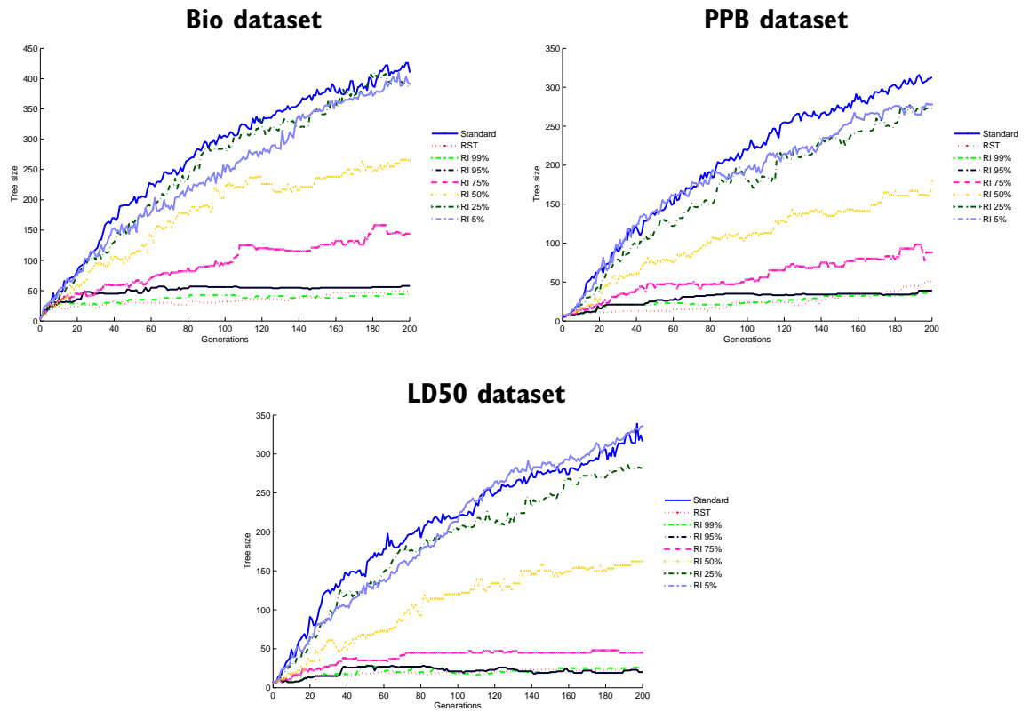
Figure 4.15: Tree size evolution plots for Standard GP, RST, and RI with different parameters
