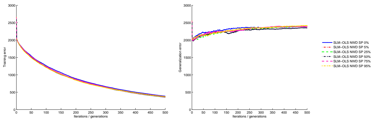
Figure 6.13: Training and generalization errors evolution plots for SLM-OLS NWD with and without sparseness
