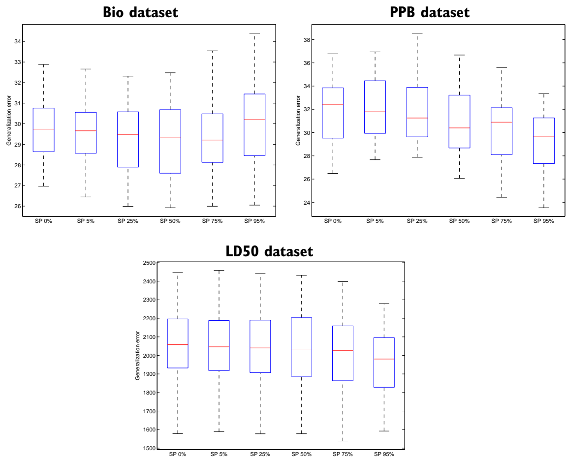
Figure 6.7: Generalization error boxplots for SLM with and without sparseness
