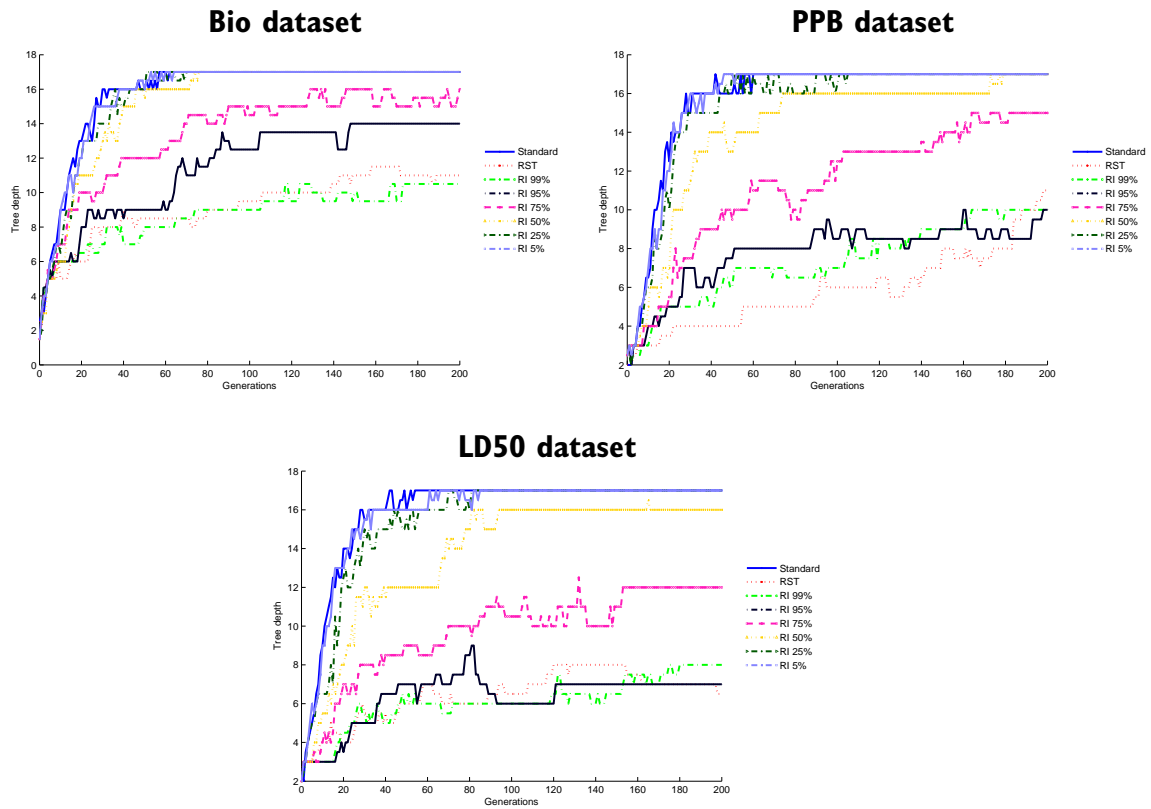
Figure 4.16: Tree depth evolution plots for Standard GP, RST, and RI with different parameters
