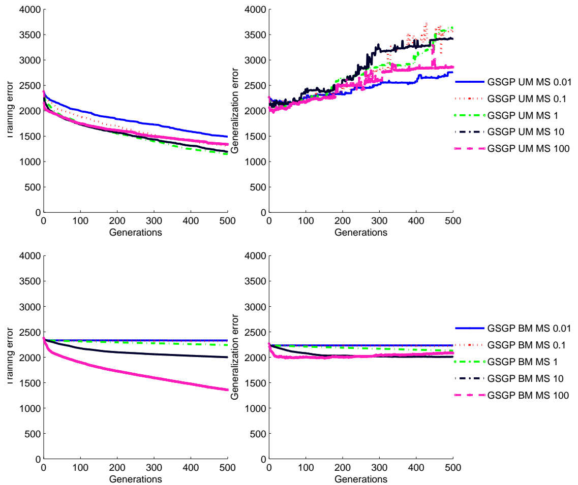
Figure 5.3: Training and generalization errors evolution plots for GSGP UM (top) and BM (bottom), with several mutation steps in the LD50 dataset
