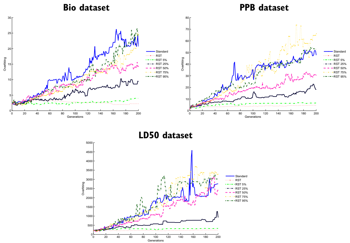
Figure 4.2: Overfitting evolution plots for Standard GP and RST with different parameters
