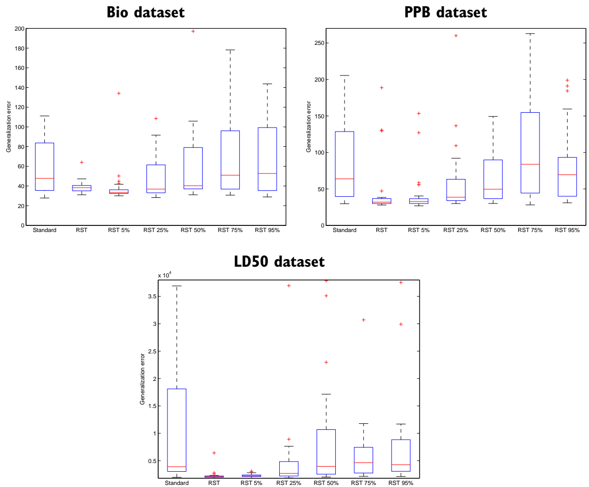
Figure 4.3: Generalization error boxplots for Standard GP and RST with different parameters
