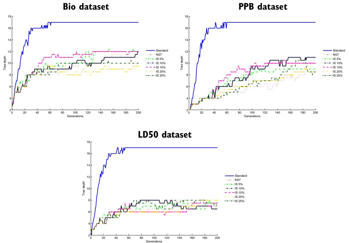
Figure 4.11: Tree depth evolution plots for Standard GP, RST, and IS with different parameters
