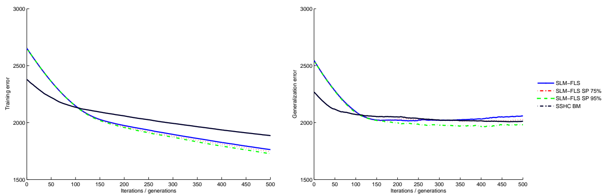
Figure 6.8: Training and generalization errors evolution plots for SLM-FLS, SLM-FLS SP 75%, SLM-FLS SP 95%, and SSHC BM
