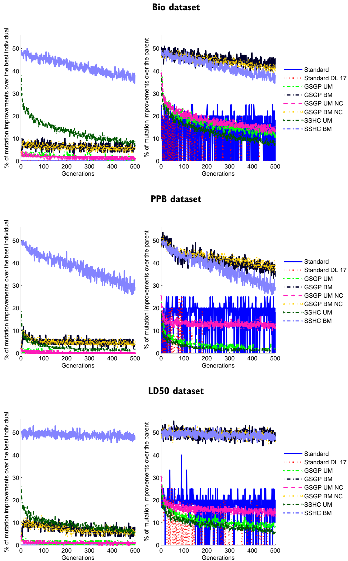
Figure 5.9: Percentage of mutation improvements for Standard GP, GSGP, and SSHC
