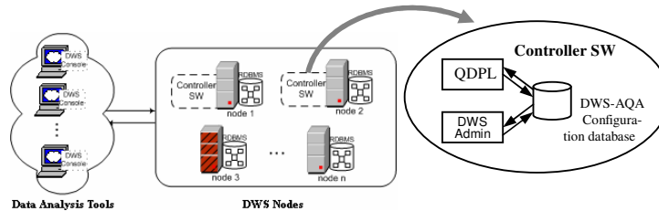
Fig. 1. A DWS-AQA cluster is composed by nodes running a DBMS and storing each one a fraction of the data warehouse partitioned according to the DWS approach. One or more nodes include the Controller SW, which is actually the DWS-AQA middle layer. The Controller SW comprises the QDPL (Query Distributed Processing Layer) the DWS Admin (Administration Tools), and a DWS Configuration Database. The DWS Configuration Database stores all the information necessary for the functioning of the DWS system and the DWS Admin is responsible for the administration of the DWS-AQA system Architecture.
