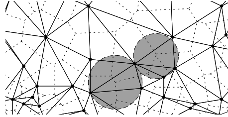
Figure 4 Delaunay Triangulation, Voronoi tessellation and the empty circumcircle property
